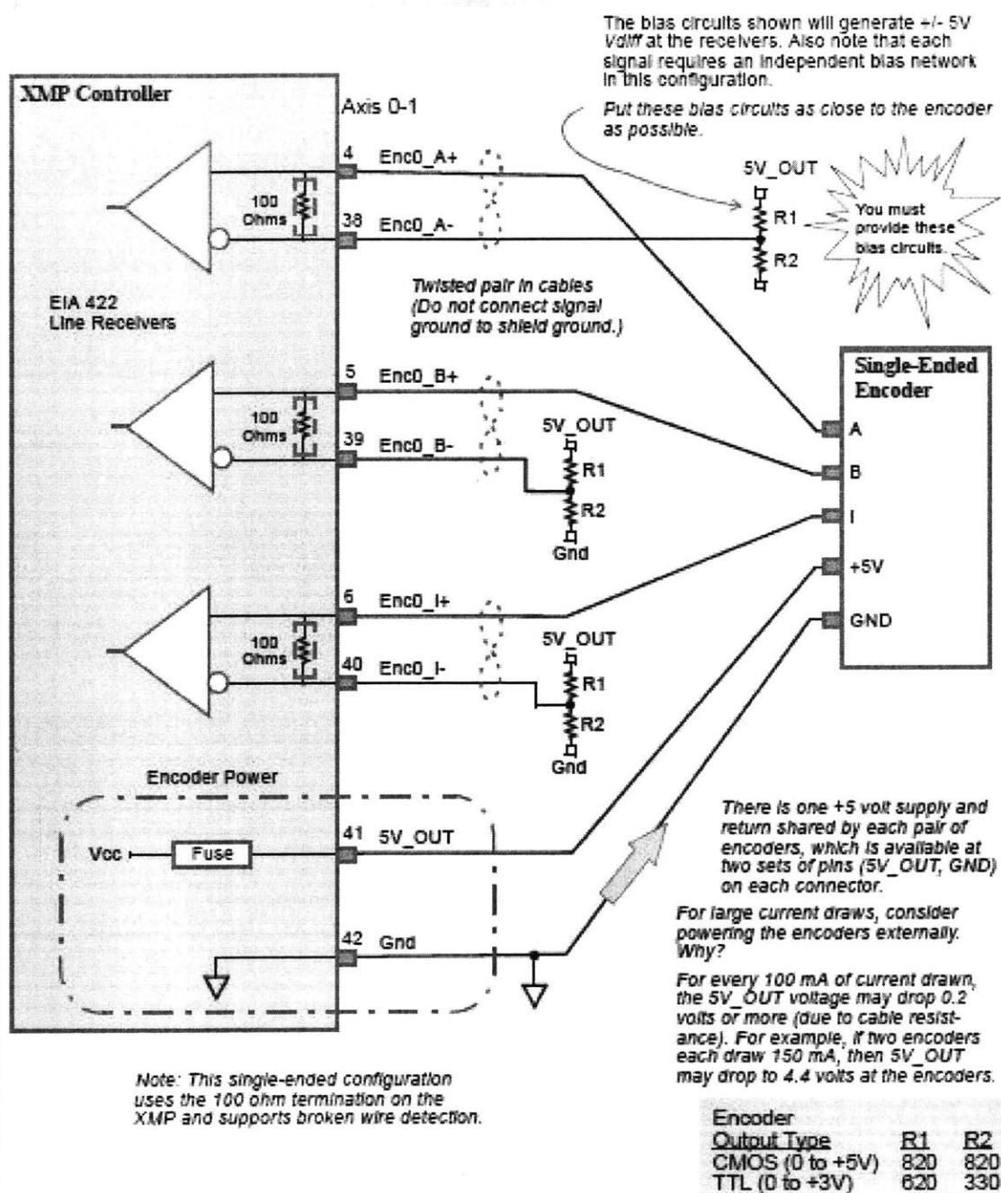
Single-Ended Encoders
