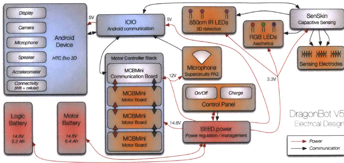
Figure 3-22: DragonBot electrical diagram
