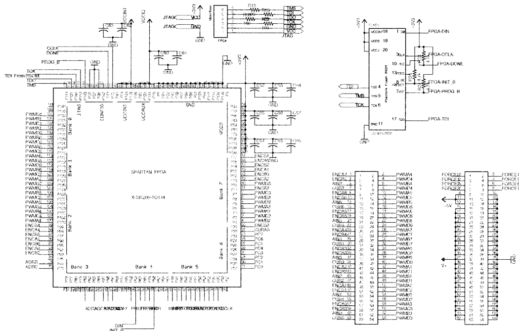
Figure 3-10: The FPGA coprocessor and its communication channels [board-to-board connectors]
