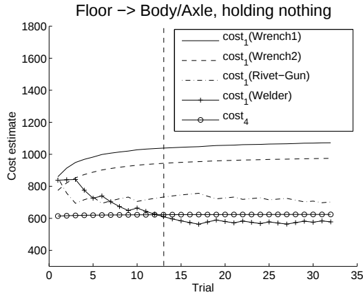
Fig. 5. Effect of an inconsistent human teammate: graph shows perceiving the Floor with an human teammate bringing the Body with a probability of 70% and an Axle with a probability of 30%.
