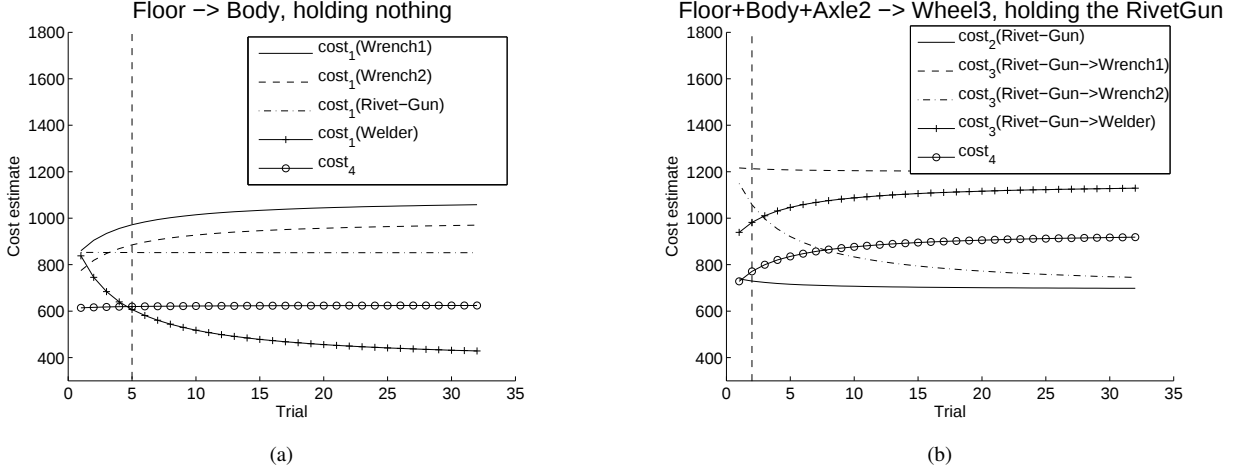
Fig. 3. Cost evaluation with a theoretical consistent human teammate. In (a) the robot is holding nothing and perceiving the Floor with a consistent human always bringing the Body next; in (b) the robot is holding the RivetGun and perceiving Floor + Body + Axle2 with a consistent human bringing Wheel3 .
