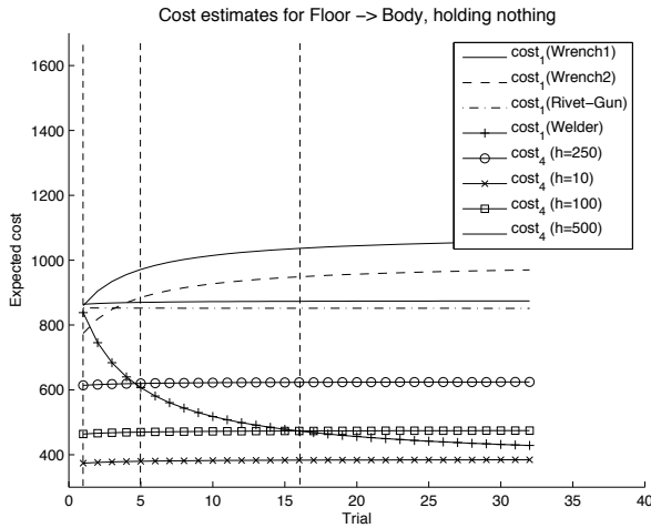
Fig. 6. Cost analysis perceiving the Floor with a consistent human teammate, but varying the estimated human turnaround cost h .
