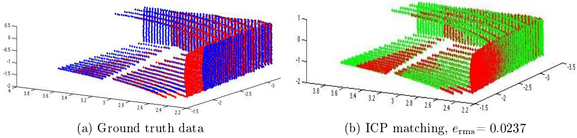
Figure 3: ICP match is very close to the ground truth
