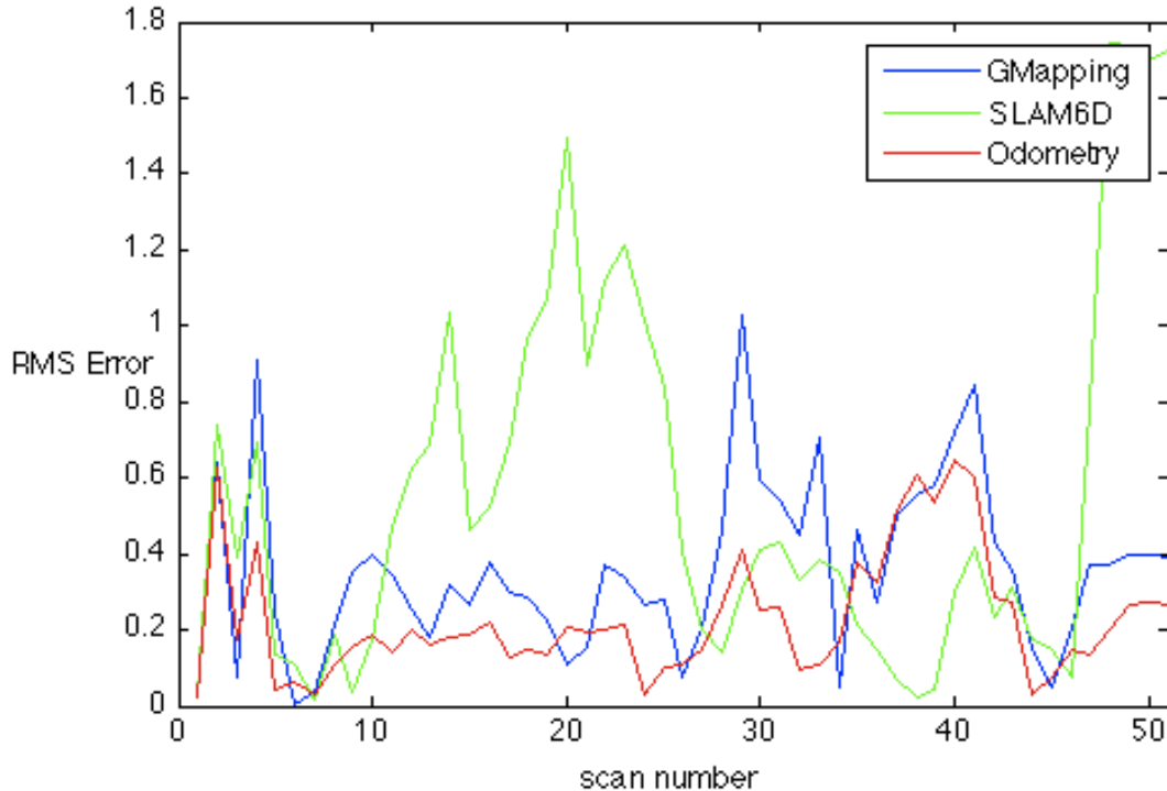
Figure 6: RMS Error.
