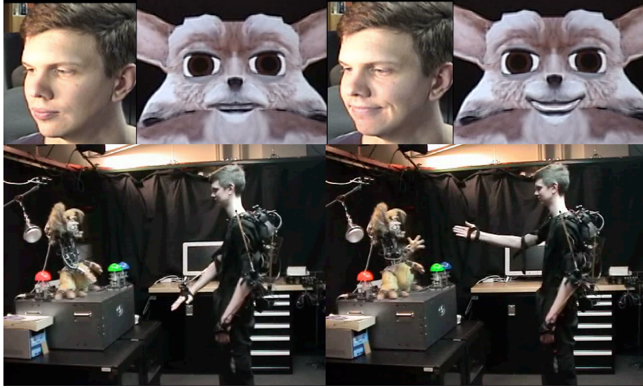
Figure 3-4: Demonstration of motor mimicry. These pictures show two different domains where the motor mapping techniques from this chapter have been demonstrated. The top row shows two human facial expressions and the resulting mimicry performed by the robot. In these examples, the output shown is the result of the process in section 3.3 - once the learning phase is over, the human’s facial points are mapped into joint angles, then those joint angles are used as an input to search the robot’s pose-graph for the closest animation (or in this case, the closest weighted blend of facial expressions animations). The bottom row shows the robot mimicking the position of the human’s arm. In this case, the direct result of the joint mapping 3.2 is being performed.
