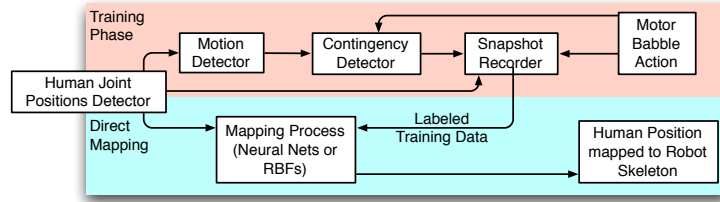
Figure 3-1: Mapping perceived human joints onto the robot’s skeleton to allow for comparison between joint configurations of robot and human. In the training phase, the robot babbles and the human imitates the robot’s pose. When the robot detects imitation (based on contingent motion timing), it saves a snapshot of the appropriate body part (a tuple of sensor data and current robot pose). Once a sufficient number of snapshots are recorded, this data can be used to create a mapping between the two spaces which is applied thereafter in realtime.
