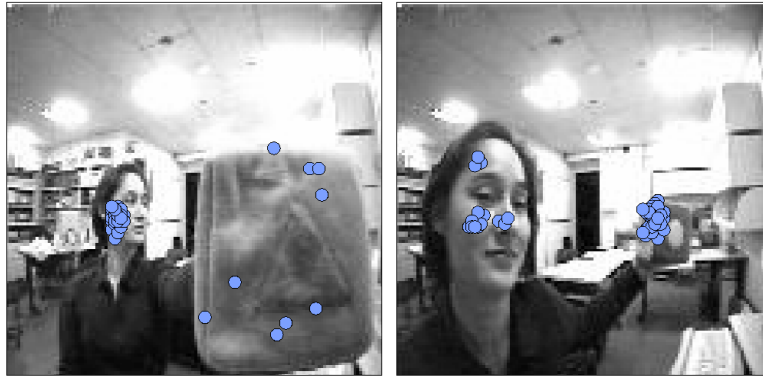
Fig. 9. Effect of gain adjustment on looking preference. Circles correspond to fixation points, sampled at one second intervals. On the left, the gain of the skin tone filter is higher. The robot spends more time looking at the face in the scene (86% face, 14% block). This bias occurs despite the fact that the face is dwarfed by the block in the visual scene. On the right, the gain of the color saliency filter is higher. The robot now spends more time looking at the brightly colored block (28% face, 72% block).
